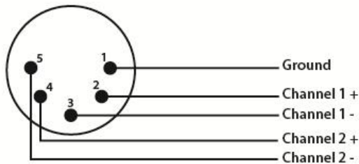
5-Pin Male XLR (rear view)
